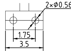
HV BUSHING TERMINAL DETAIL
