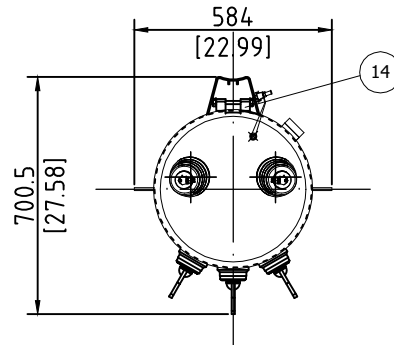
GROUNDING COUNECTOR DETAIL
